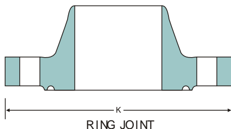
RING JOINT
