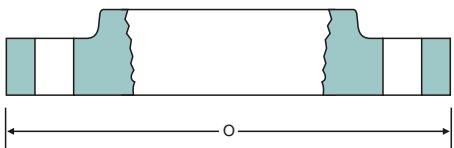
FLAT FACE
