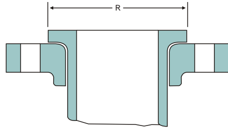
LAPPED JOINT
