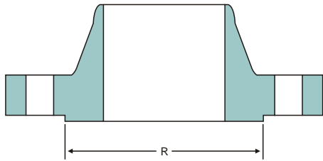
RAISED FACE
