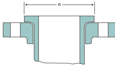
LAPPED JOINT
